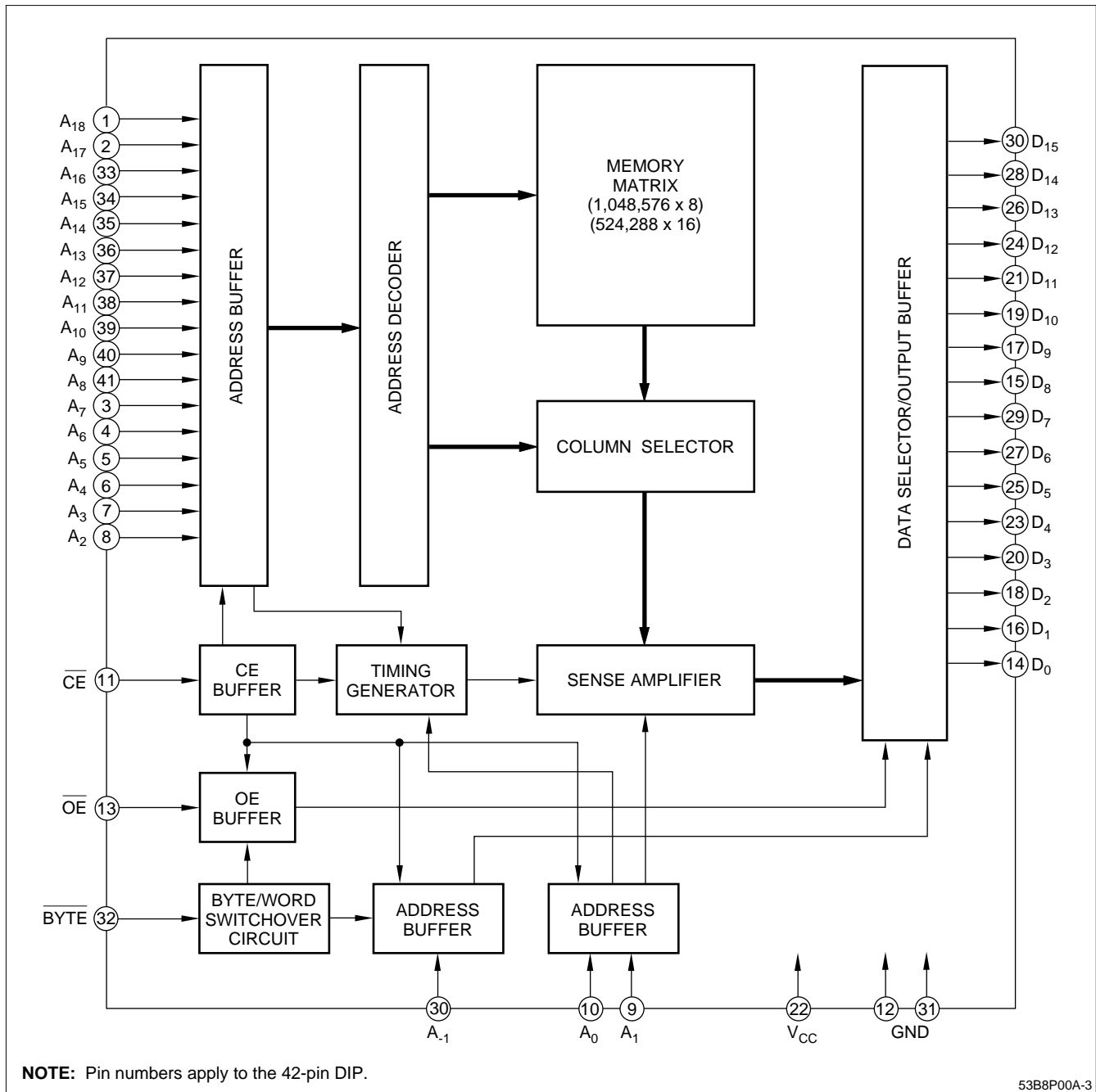
Figure 3. LH53B8P00A Block Diagram
